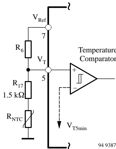
Figure 14. Temperature comparator
