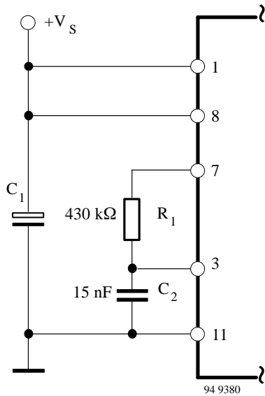
Figure 6. 200-Hz oscillator
